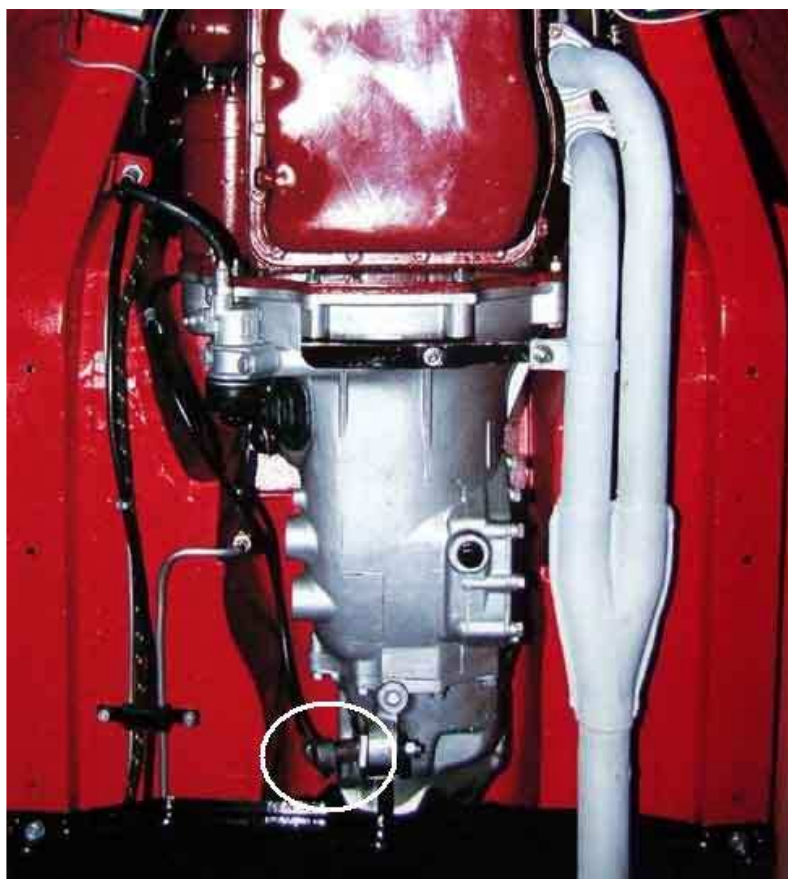
1974 LHD car from Clausager, showing (probably) how the speedo cable and heat control cable exit the bulkhead
